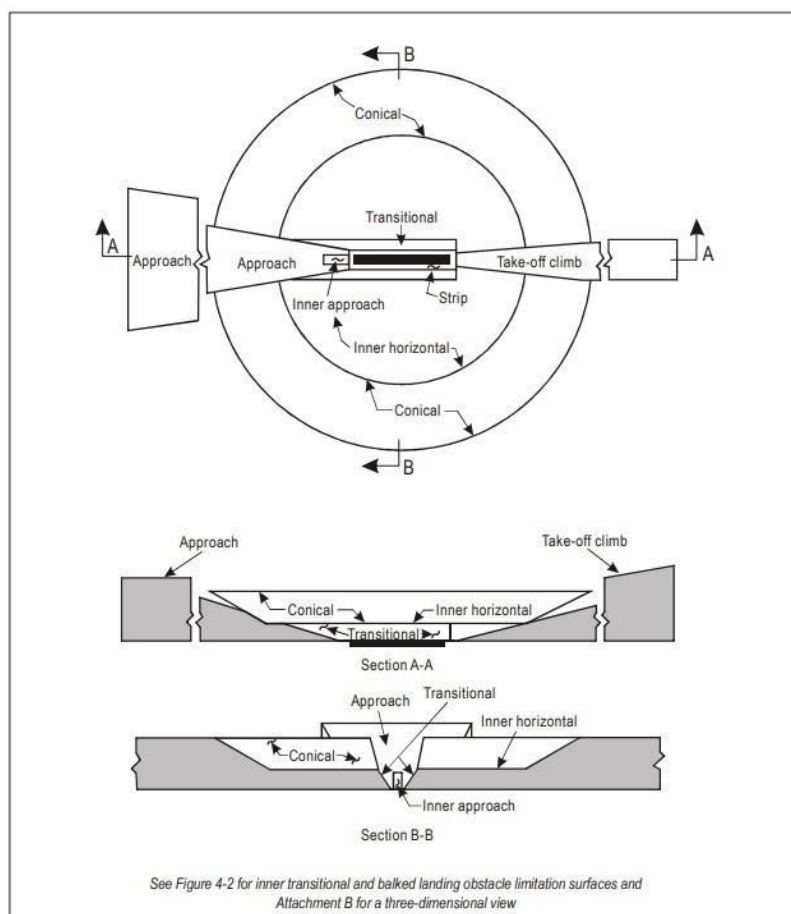
Figure 3: ICAO Obstacle Limitation Surfaces
